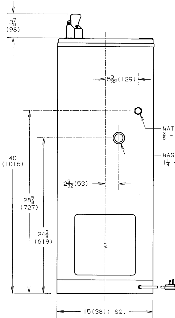
REAR VIEW
